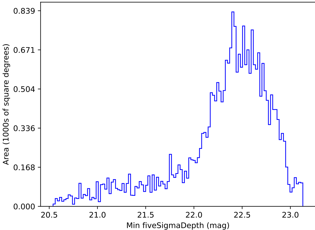
too_elab_r8_d3_giz_v3.4_10yrs Yr 1 z band: Min fiveSigmaDepth
