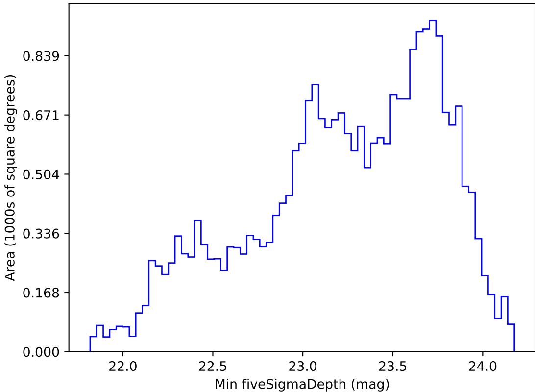
too_elab_r8_d3_giz_v3.4_10yrs Yr 1 r band: Min fiveSigmaDepth
