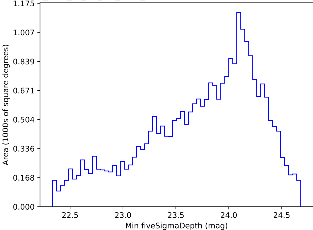
too_elab_r8_d3_giz_v3.4_10yrs Yr 1 g band: Min fiveSigmaDepth
