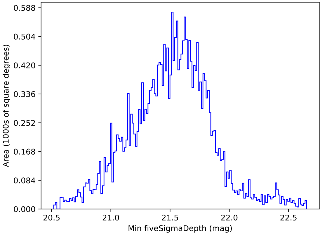
too_elab_r8_d3_giz_v3.4_10yrs Yr 1 all bands: Min fiveSigmaDepth
