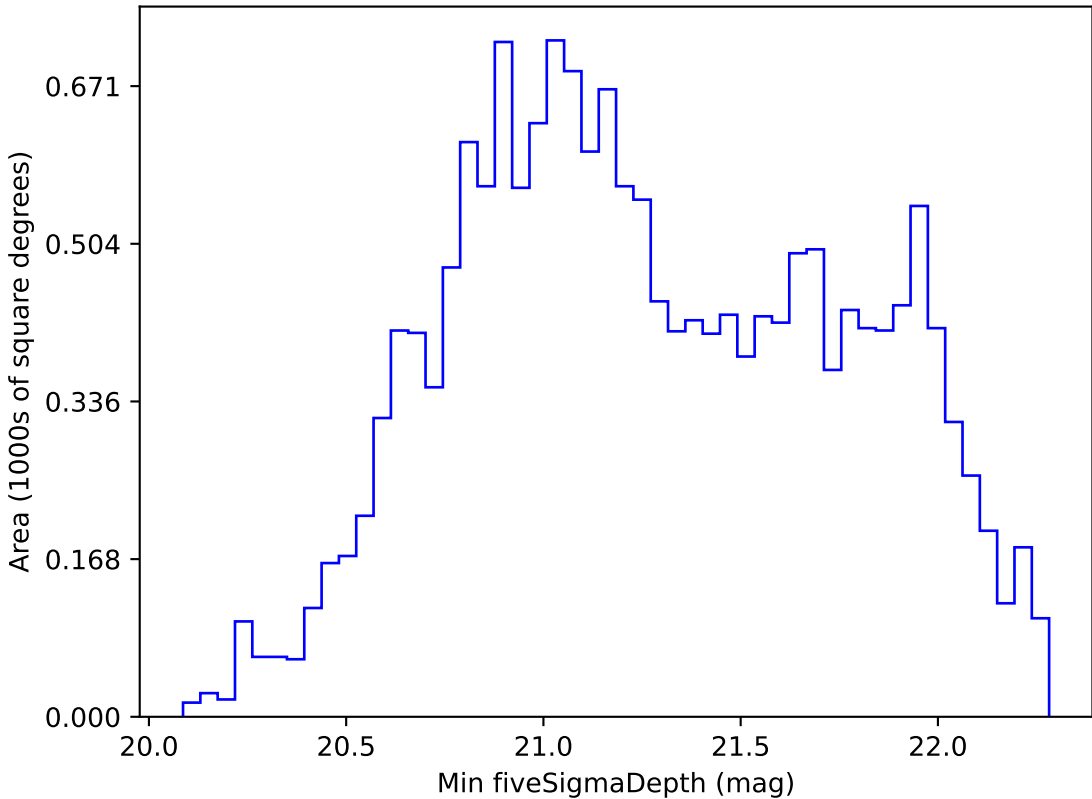
too_elab_r8_d3_giz_v3.4_10yrs WFD z band: Min fiveSigmaDepth
