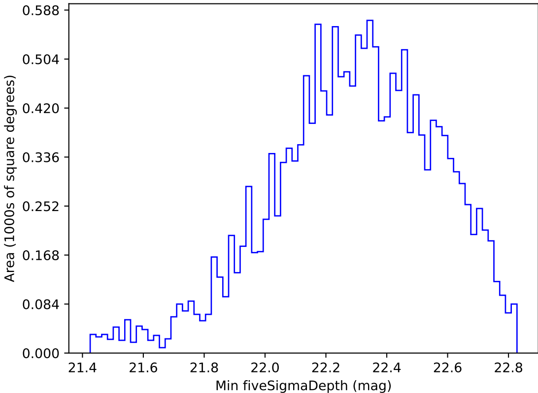
too_elab_r8_d3_giz_v3.4_10yrs WFD u band: Min fiveSigmaDepth
