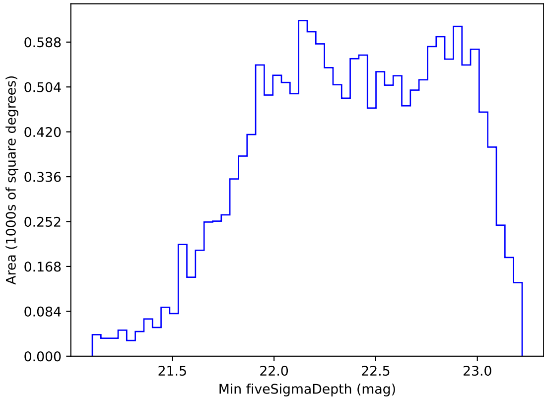
too_elab_r8_d3_giz_v3.4_10yrs WFD r band: Min fiveSigmaDepth
