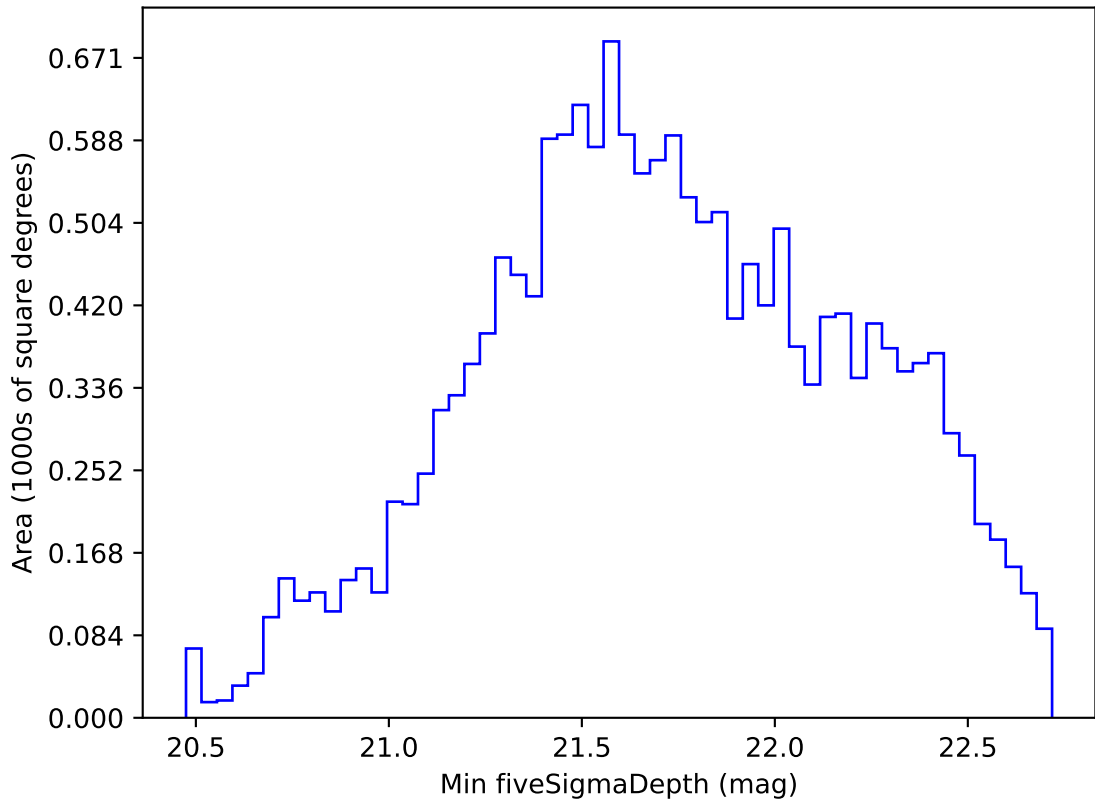
too_elab_r8_d3_giz_v3.4_10yrs WFD i band: Min fiveSigmaDepth
