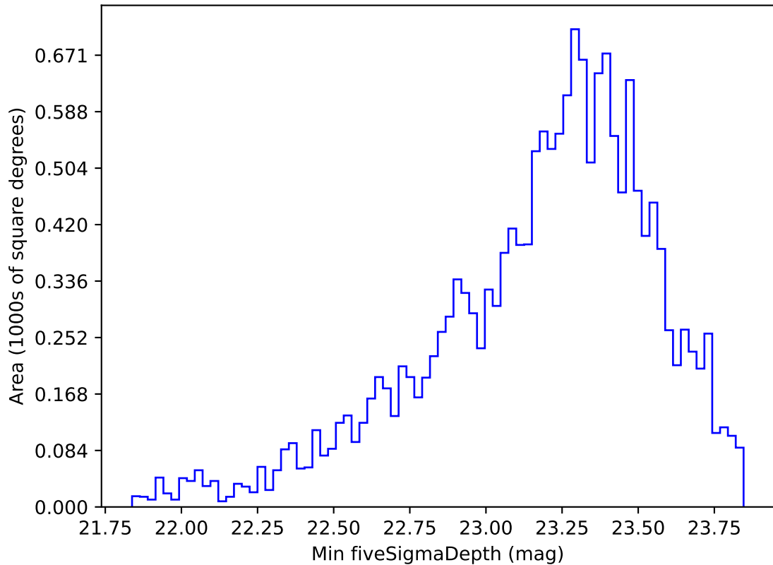
too_elab_r8_d3_giz_v3.4_10yrs WFD g band: Min fiveSigmaDepth
