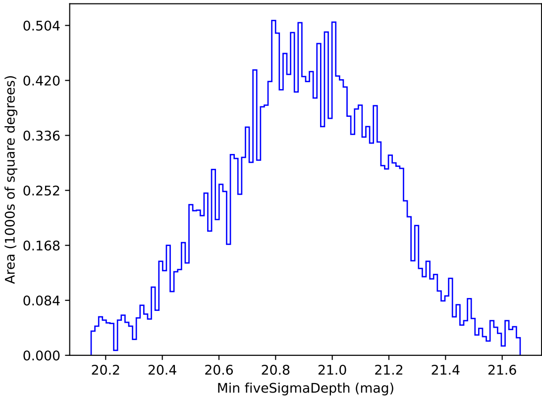
too_elab_r8_d3_giz_v3.4_10yrs All sky y band: Min fiveSigmaDepth
