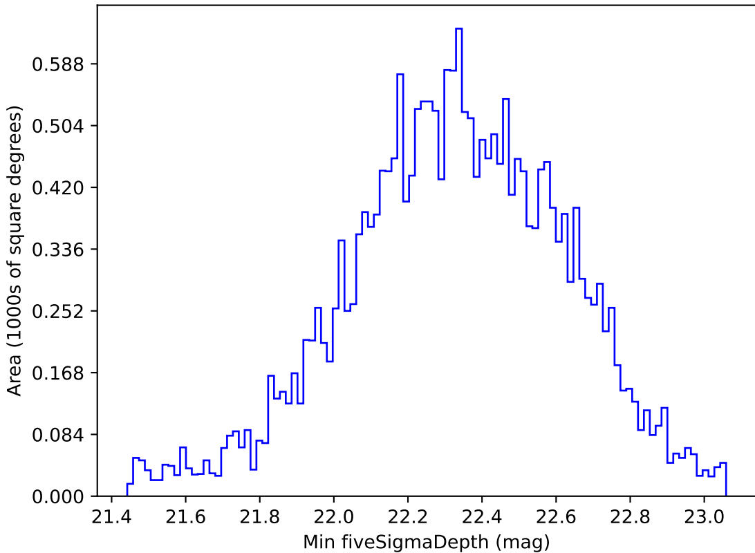
too_elab_r8_d3_giz_v3.4_10yrs All sky u band: Min fiveSigmaDepth
