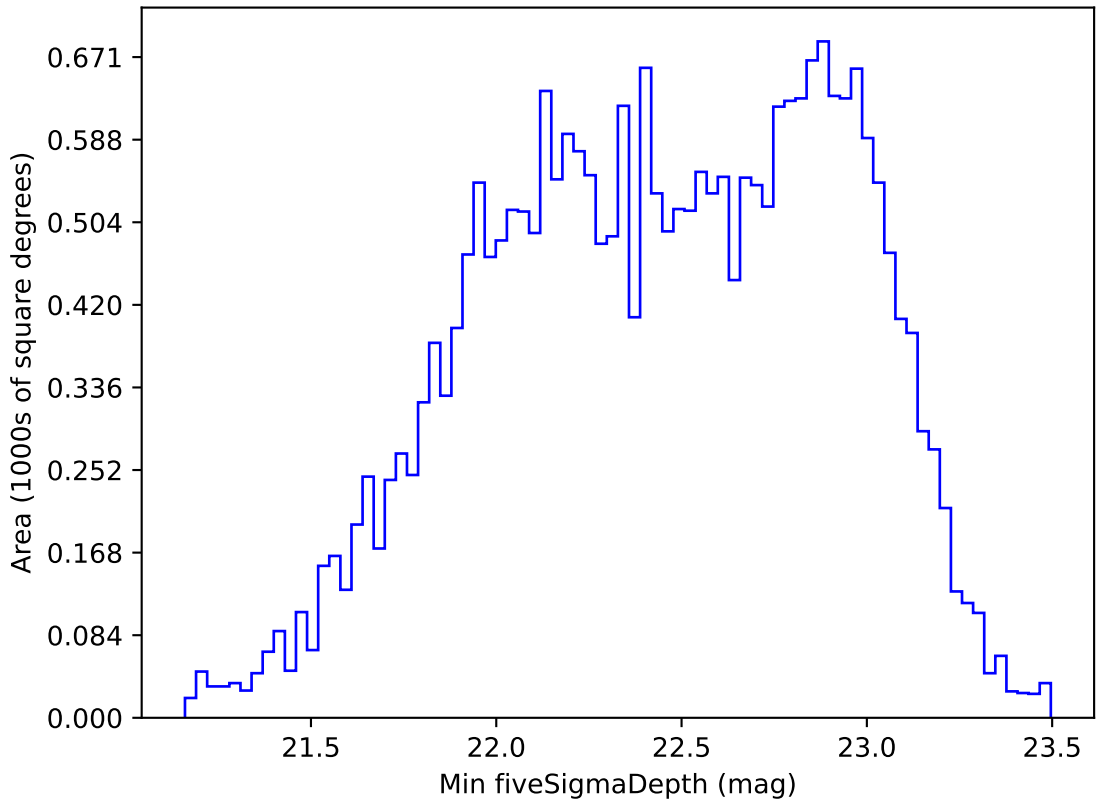
too_elab_r8_d3_giz_v3.4_10yrs All sky r band: Min fiveSigmaDepth
