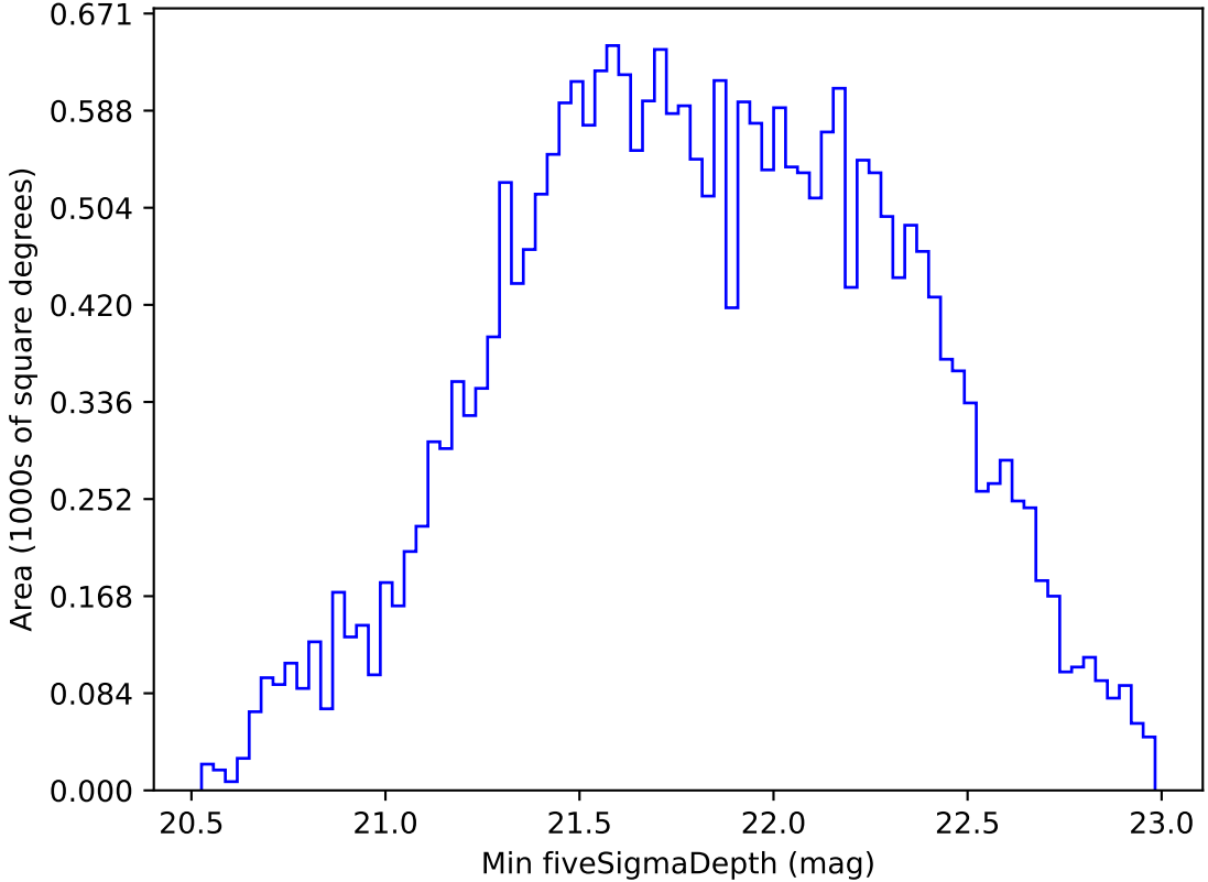
too_elab_r8_d3_giz_v3.4_10yrs All sky i band: Min fiveSigmaDepth
