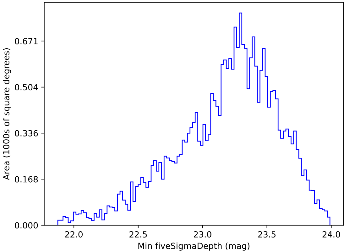
too_elab_r8_d3_giz_v3.4_10yrs All sky g band: Min fiveSigmaDepth
