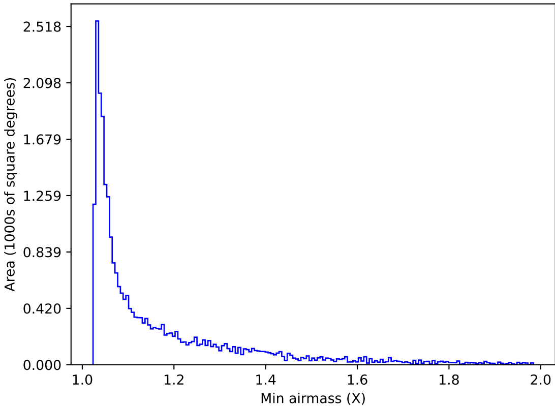
too_elab_r8_d3_giz_v3.4_10yrs Yr 1 z band: Min airmass
