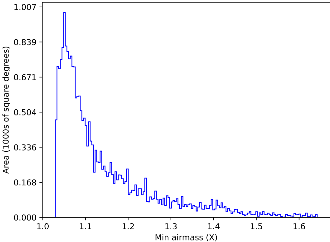
too_elab_r8_d3_giz_v3.4_10yrs Yr 1 u band: Min airmass
