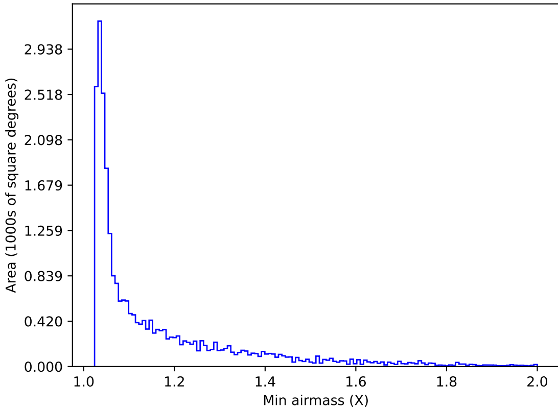
too_elab_r8_d3_giz_v3.4_10yrs Yr 1 r band: Min airmass
