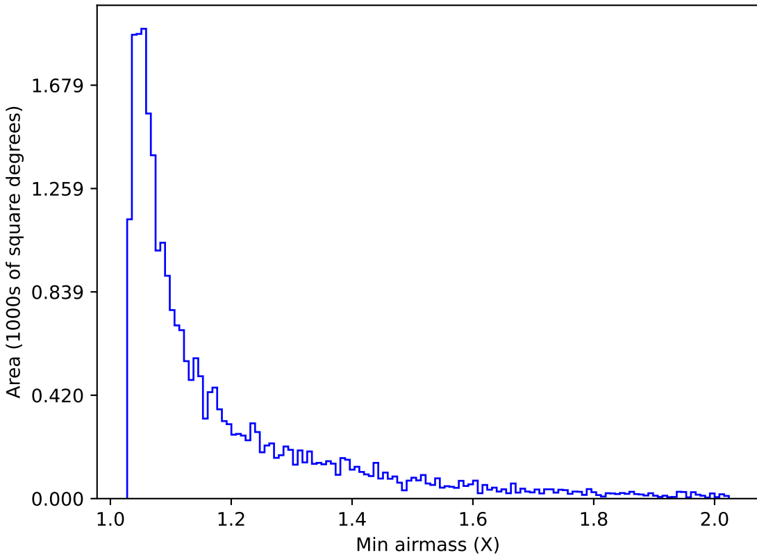
too_elab_r8_d3_giz_v3.4_10yrs Yr 1 g band: Min airmass
