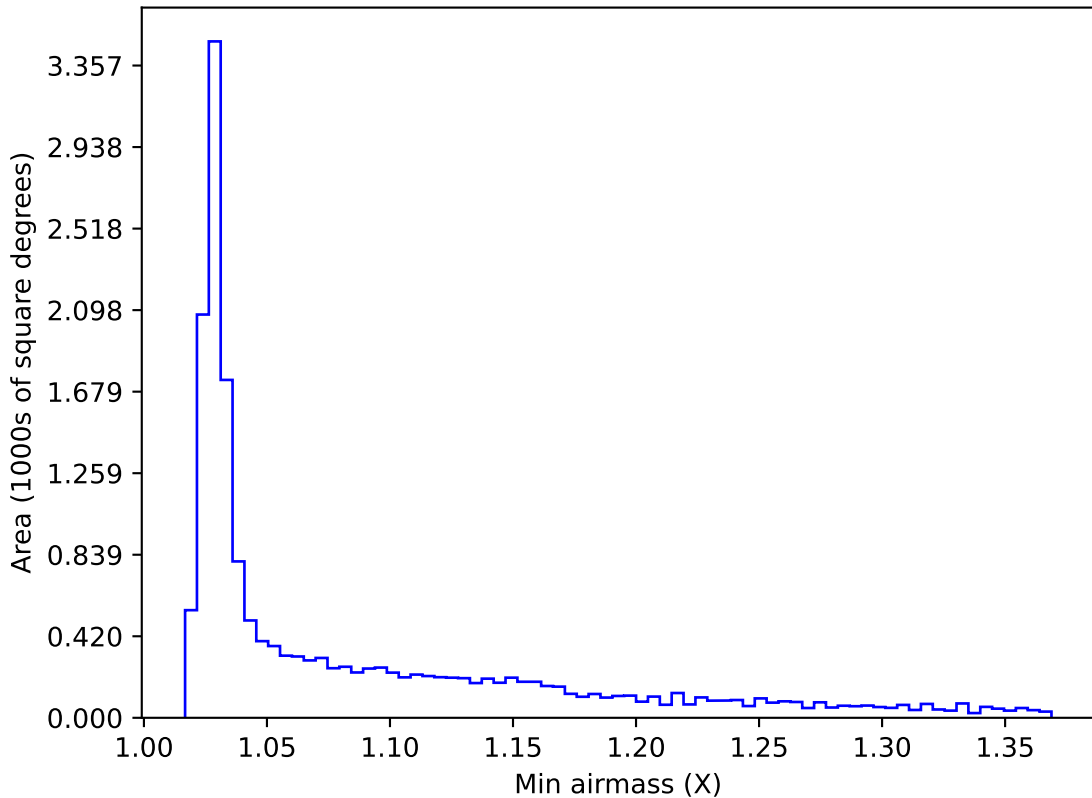
too_elab_r8_d3_giz_v3.4_10yrs WFD z band: Min airmass
