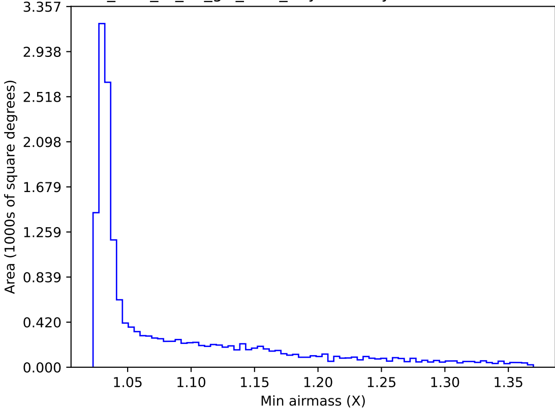
too_elab_r8_d3_giz_v3.4_10yrs WFD y band: Min airmass
