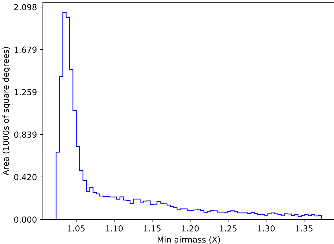
too_elab_r8_d3_giz_v3.4_10yrs WFD u band: Min airmass
