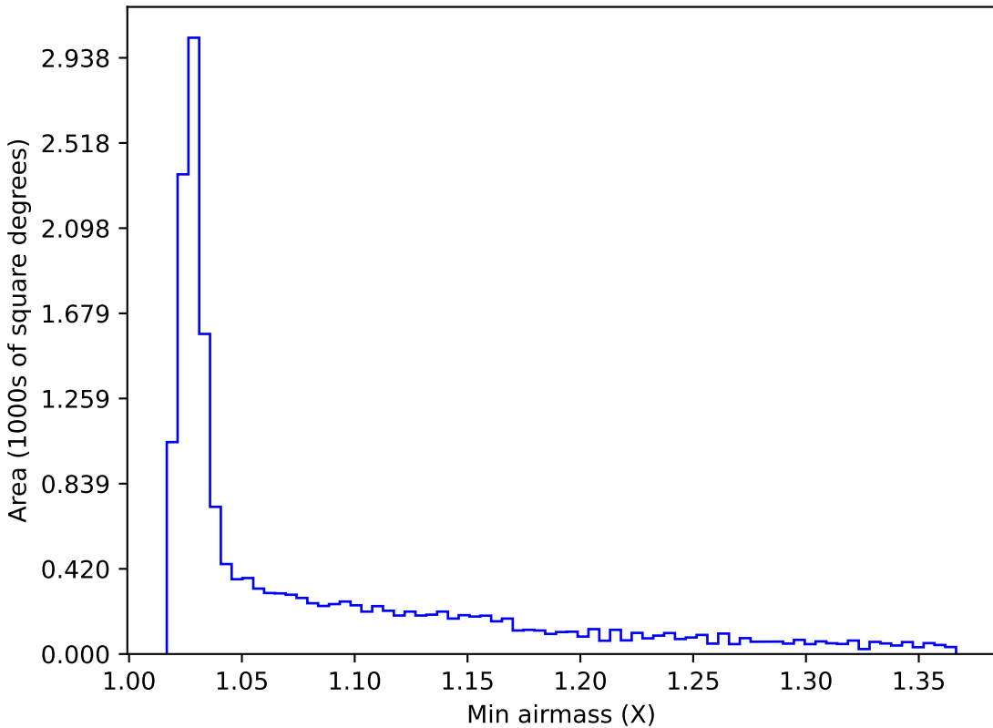
too_elab_r8_d3_giz_v3.4_10yrs WFD r band: Min airmass
