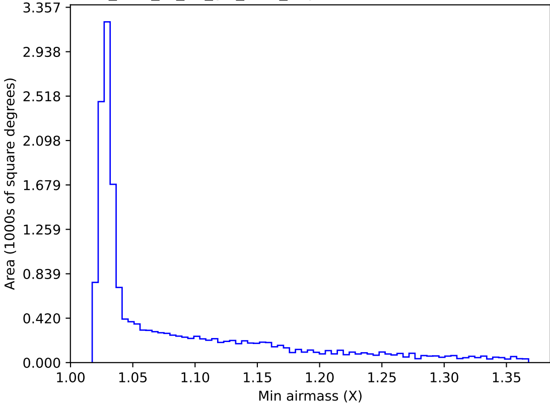
too_elab_r8_d3_giz_v3.4_10yrs WFD i band: Min airmass
