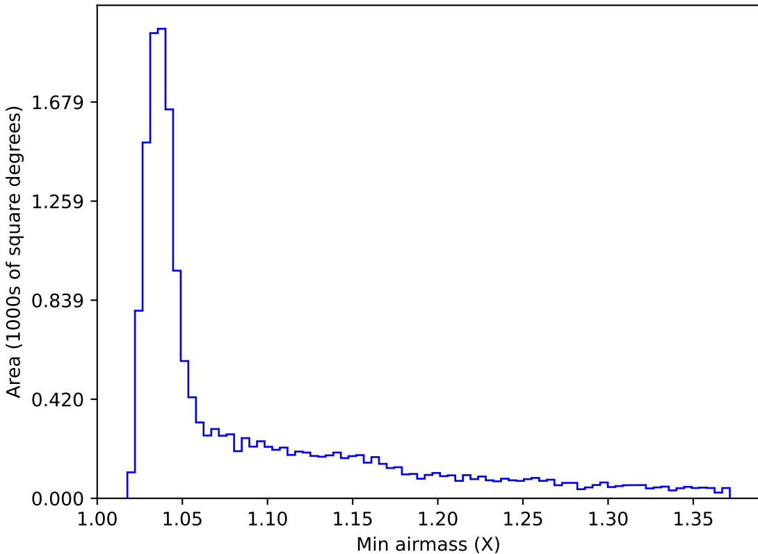
too_elab_r8_d3_giz_v3.4_10yrs WFD g band: Min airmass
