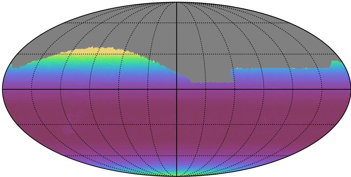
too_elab_r8_d3_giz_v3.4_10yrs All sky z band: Min airmass
