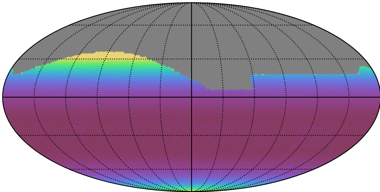
too_elab_r8_d3_giz_v3.4_10yrs All sky r band: Min airmass
