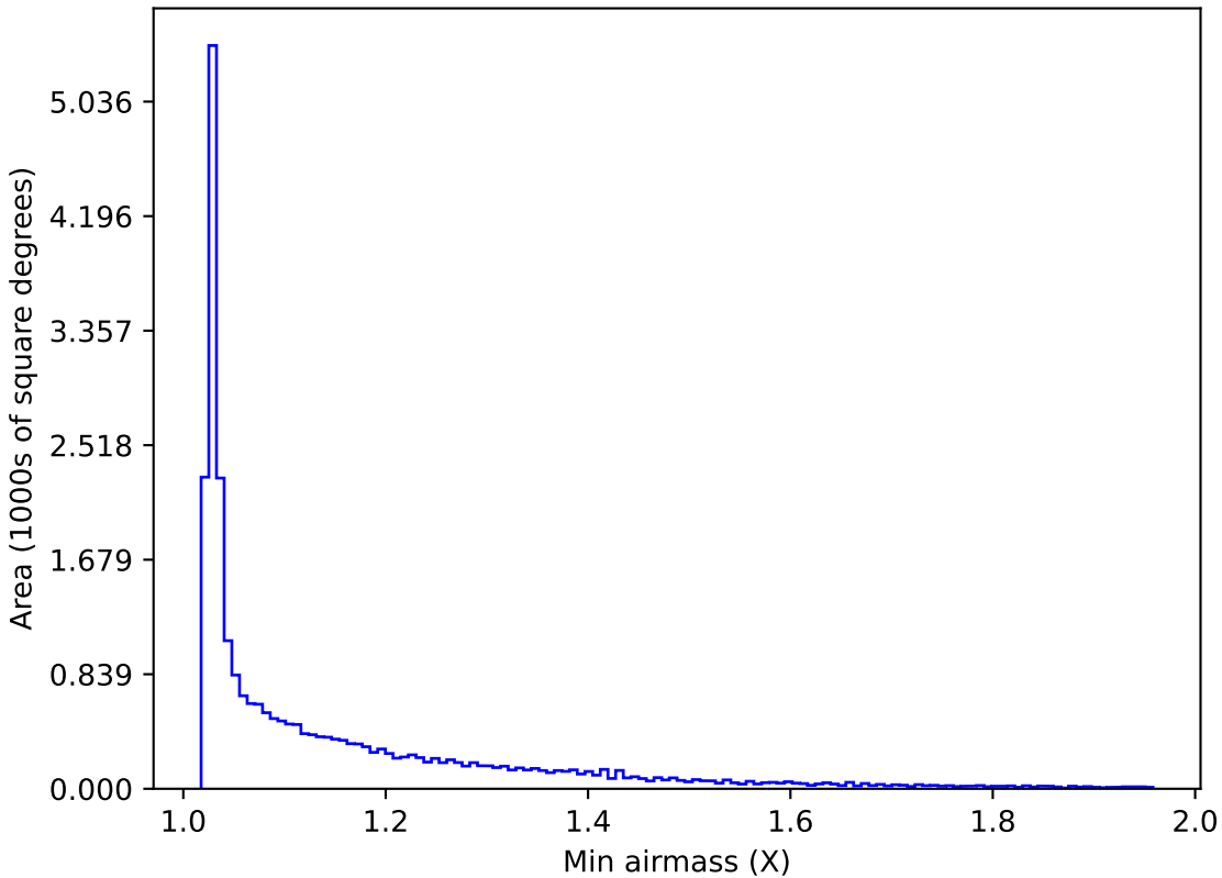
too_elab_r8_d3_giz_v3.4_10yrs All sky i band: Min airmass
