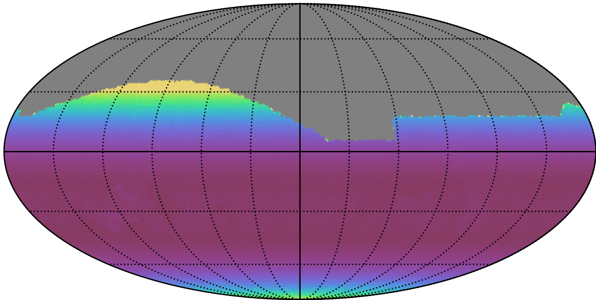
too_elab_r8_d3_giz_v3.4_10yrs All sky g band: Min airmass
