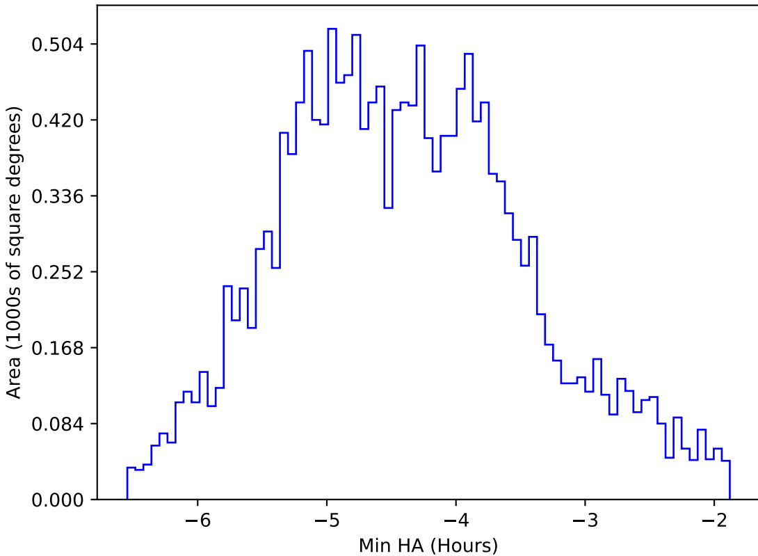
too_elab_r8_d3_giz_v3.4_10yrs WFD z band: Min HA
