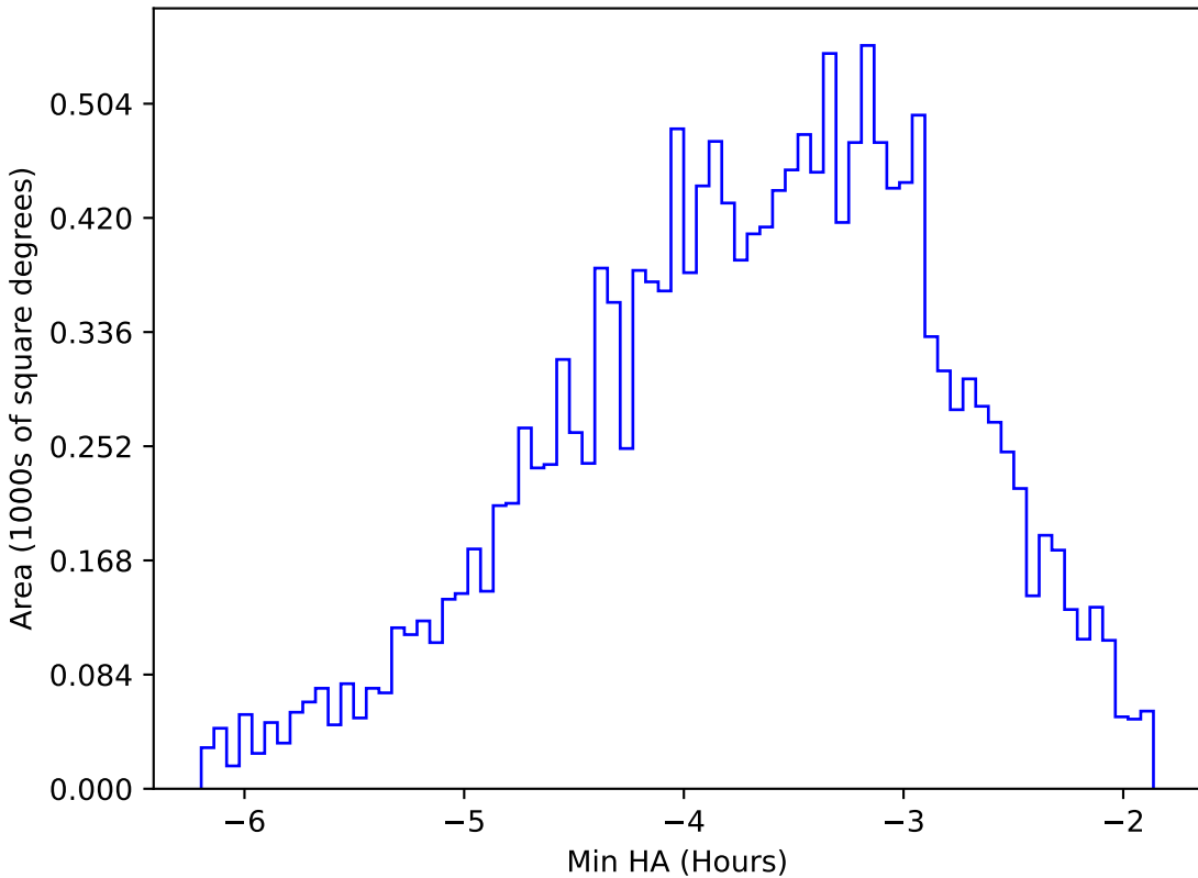
too_elab_r8_d3_giz_v3.4_10yrs WFD y band: Min HA
