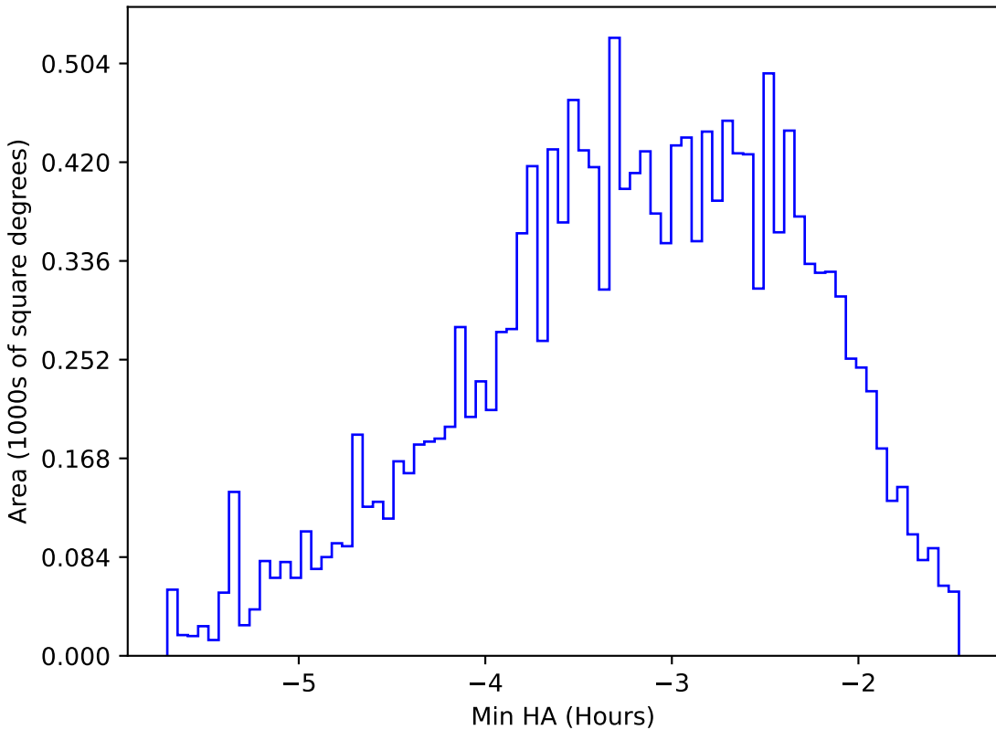
too_elab_r8_d3_giz_v3.4_10yrs WFD u band: Min HA
