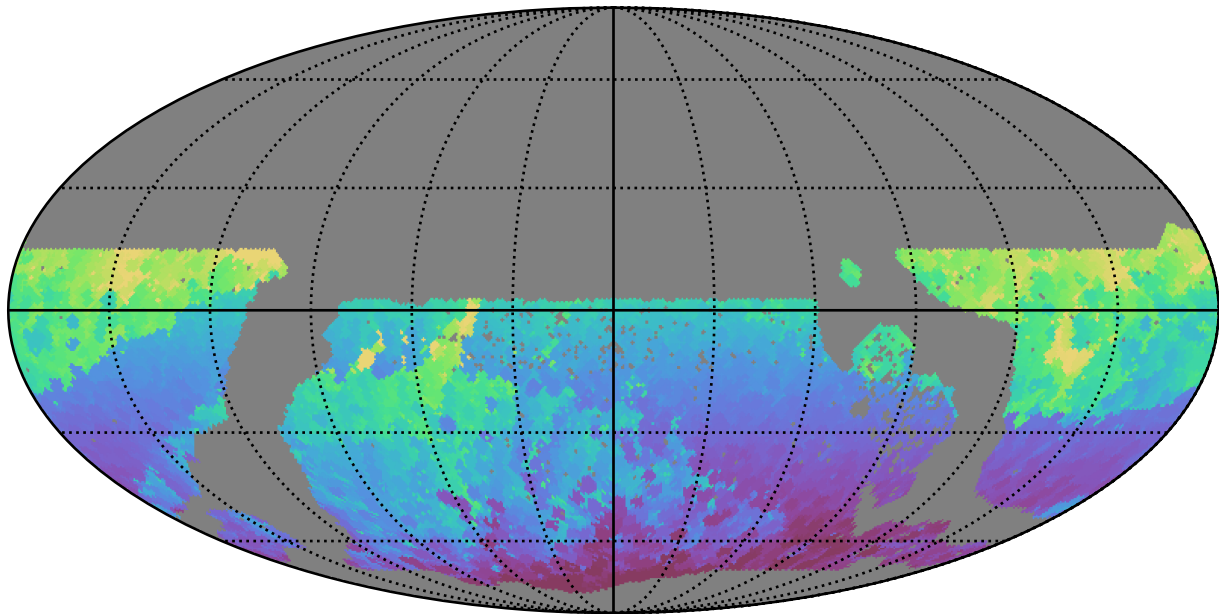
too_elab_r8_d3_giz_v3.4_10yrs WFD r band: Min HA
