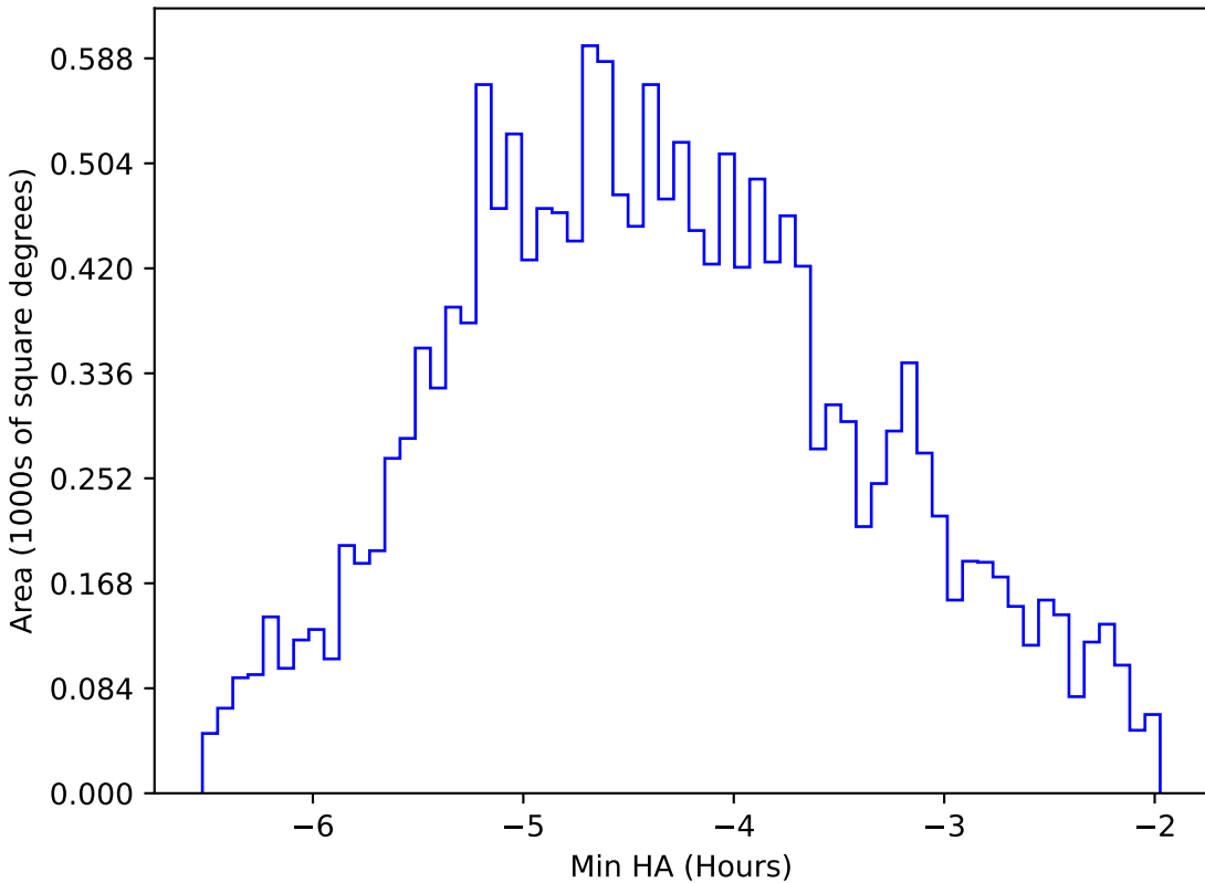
too_elab_r8_d3_giz_v3.4_10yrs WFD i band: Min HA
