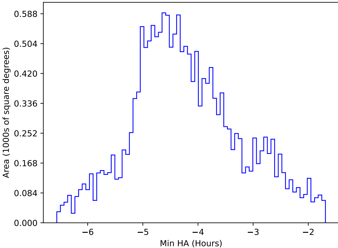
too_elab_r8_d3_giz_v3.4_10yrs WFD g band: Min HA
