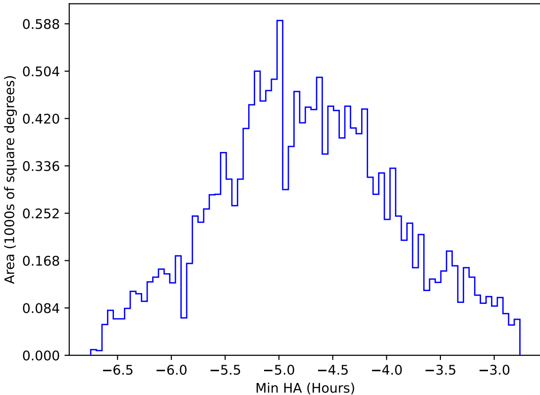
too_elab_r8_d3_giz_v3.4_10yrs WFD all bands: Min HA
