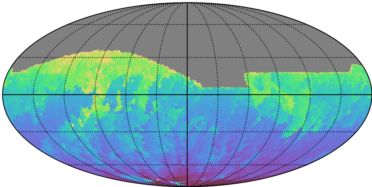
too_elab_r8_d3_giz_v3.4_10yrs All sky z band: Min HA
