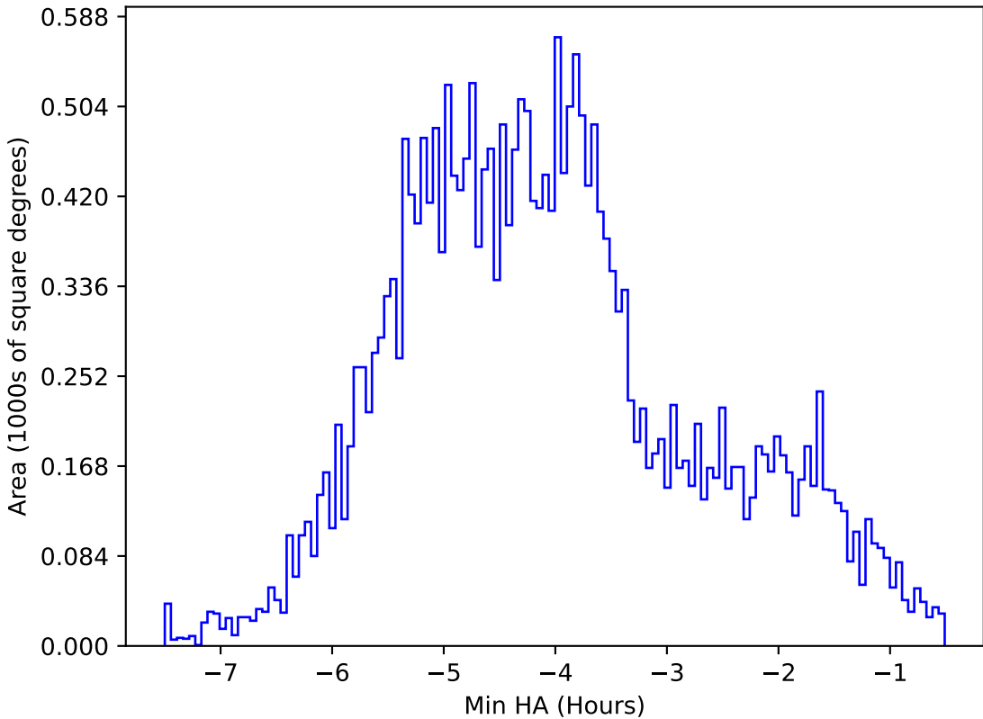
too_elab_r8_d3_giz_v3.4_10yrs All sky z band: Min HA
