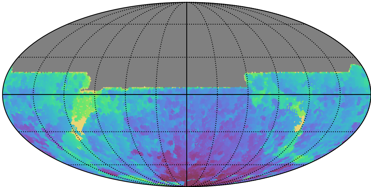
too_elab_r8_d3_giz_v3.4_10yrs All sky y band: Min HA
