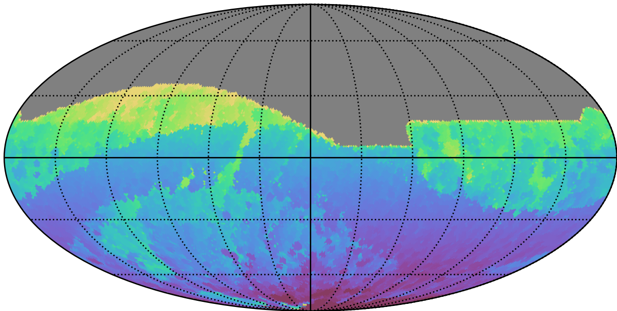
too_elab_r8_d3_giz_v3.4_10yrs All sky r band: Min HA
