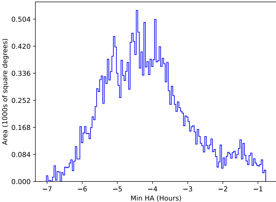
too_elab_r8_d3_giz_v3.4_10yrs All sky r band: Min HA
