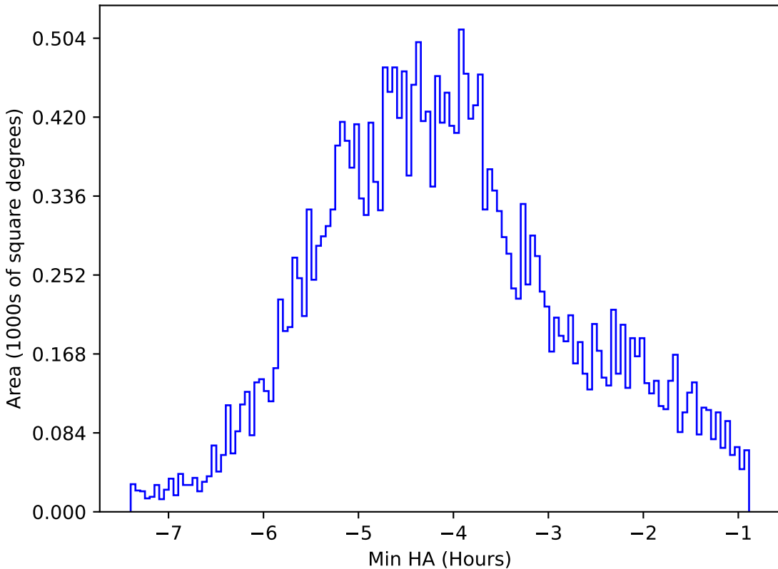
too_elab_r8_d3_giz_v3.4_10yrs All sky i band: Min HA
