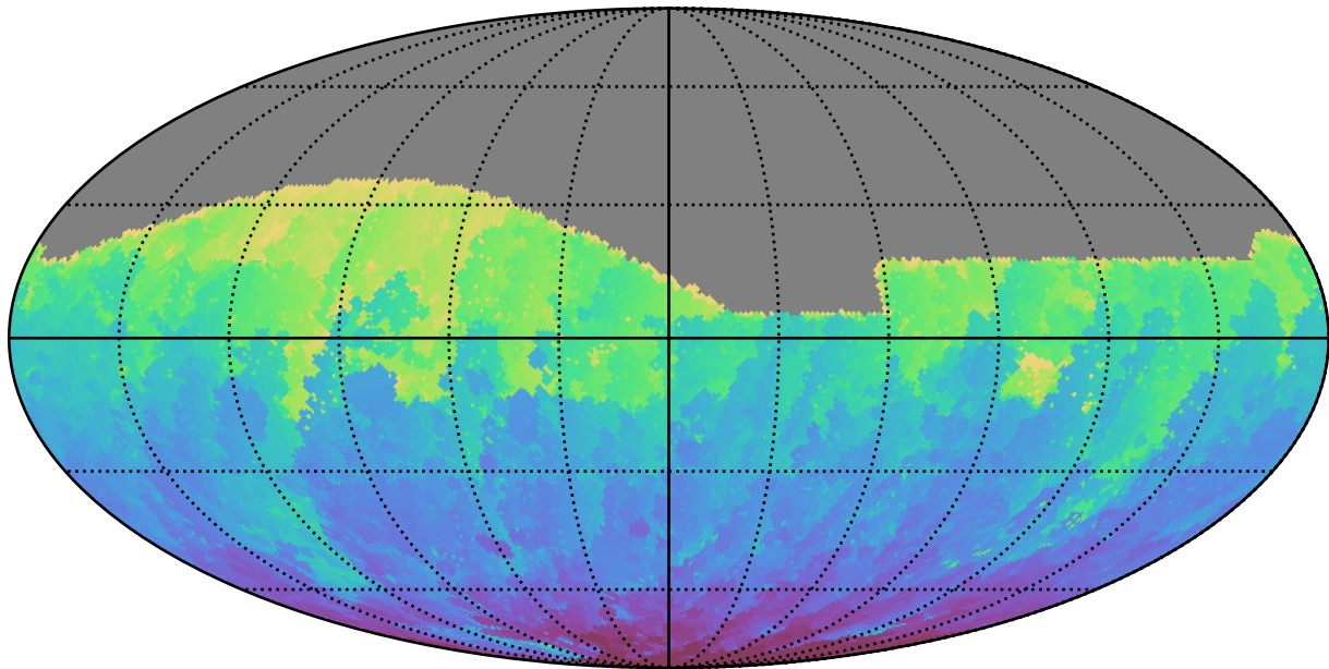
too_elab_r8_d3_giz_v3.4_10yrs All sky g band: Min HA
