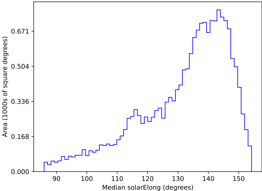
too_elab_r8_d3_giz_v3.4_10yrs WFD u band: Median solarElong
