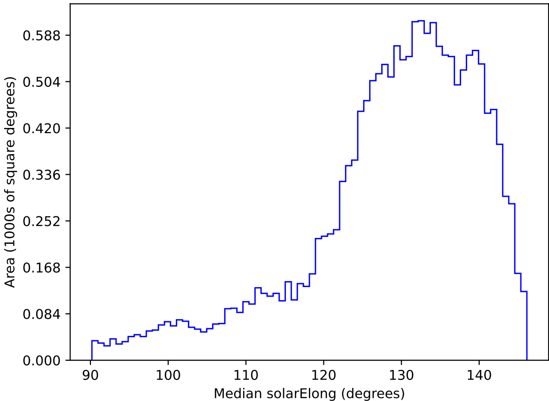
too_elab_r8_d3_giz_v3.4_10yrs WFD i band: Median solarElong
