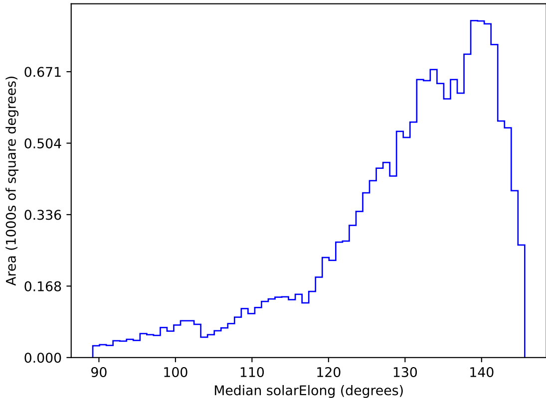
too_elab_r8_d3_giz_v3.4_10yrs WFD all bands: Median solarElong
