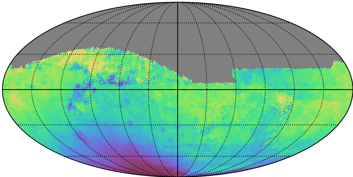
too_elab_r8_d3_giz_v3.4_10yrs All sky z band: Median solarElong
