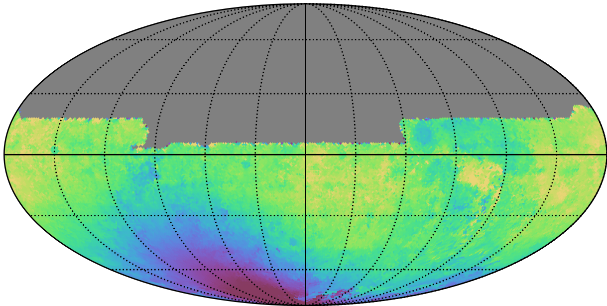
too_elab_r8_d3_giz_v3.4_10yrs All sky y band: Median solarElong
