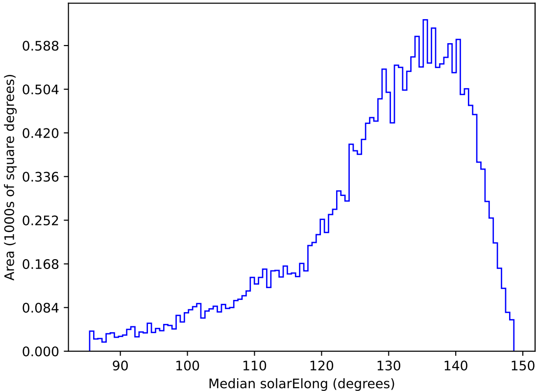
too_elab_r8_d3_giz_v3.4_10yrs All sky y band: Median solarElong
