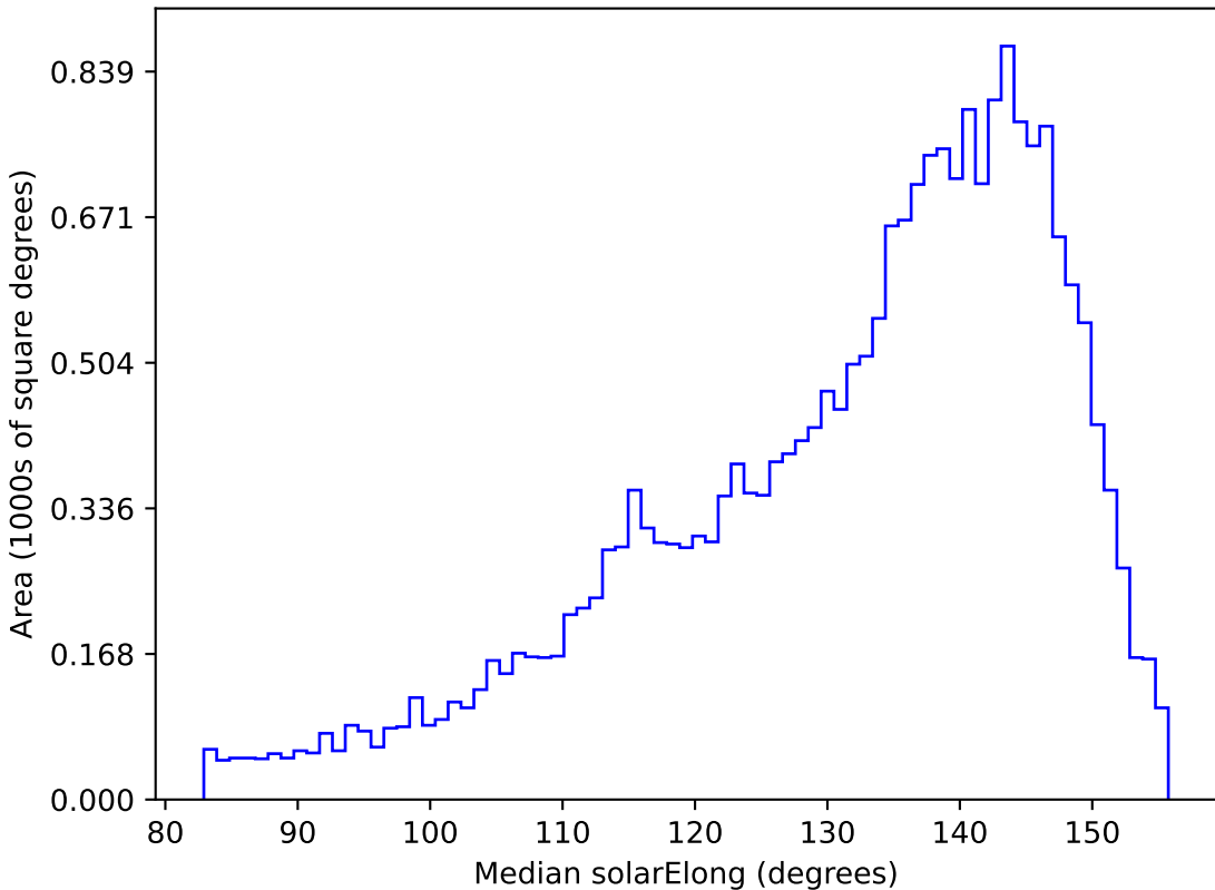
too_elab_r8_d3_giz_v3.4_10yrs All sky u band: Median solarElong
