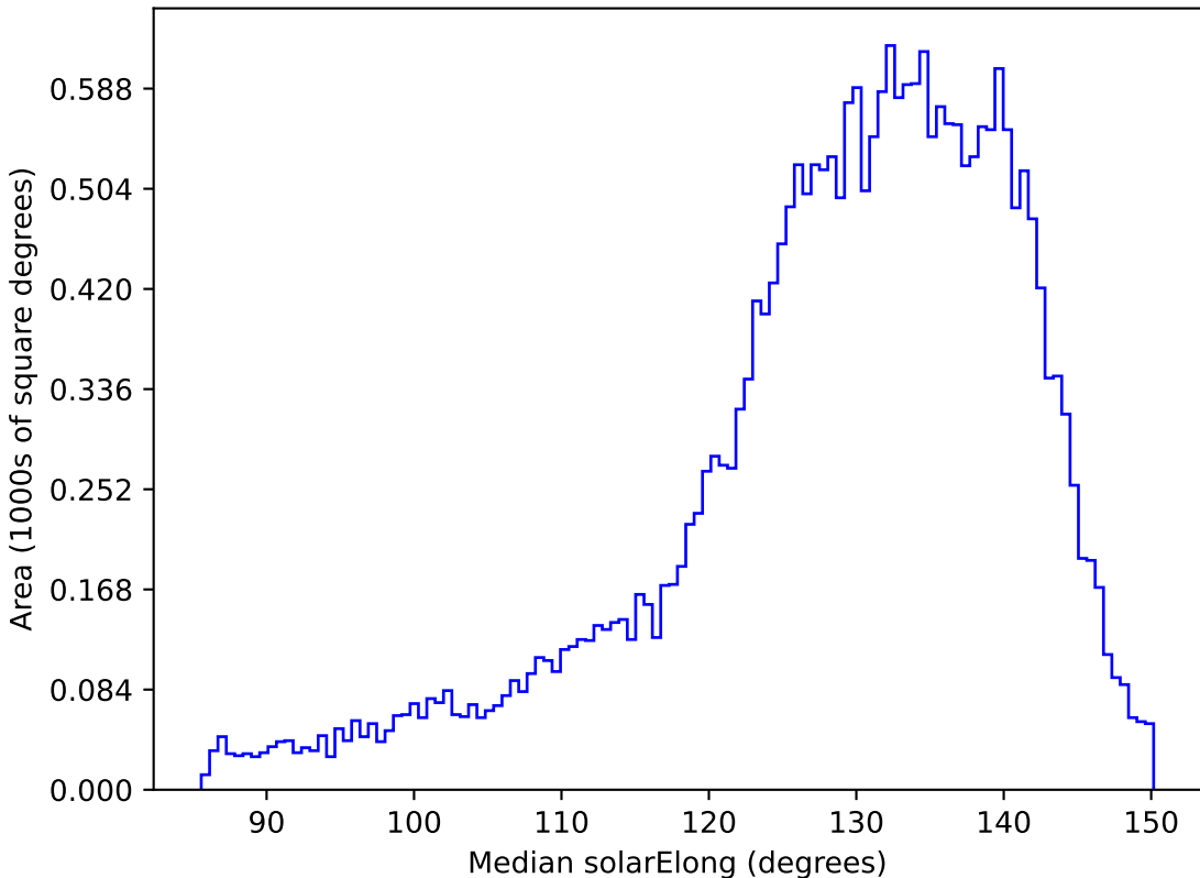
too_elab_r8_d3_giz_v3.4_10yrs All sky i band: Median solarElong
